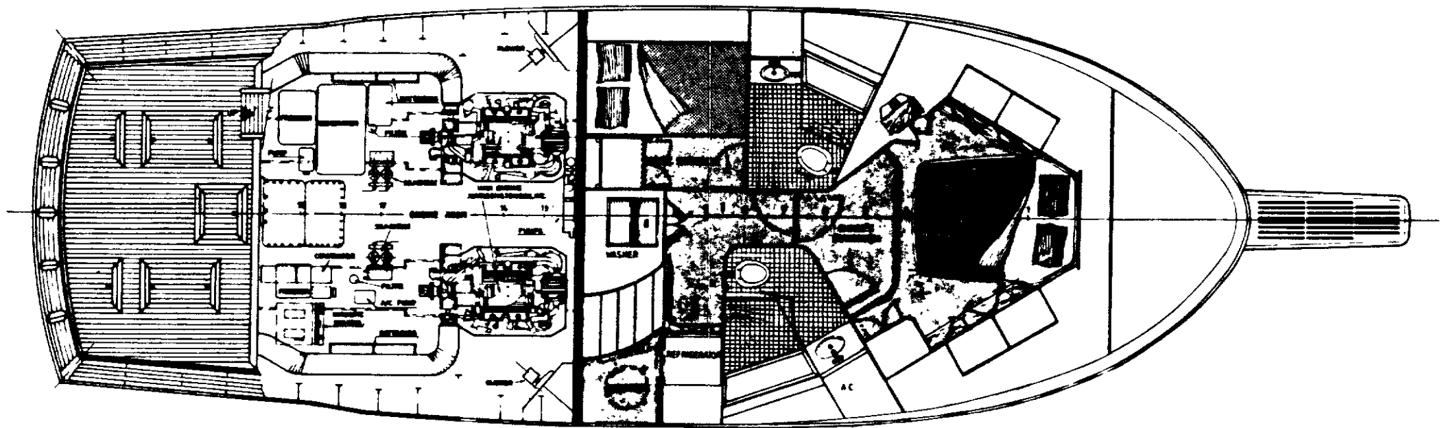
PARTIAL ARRANGEMENT AND ENGINE ROOM
