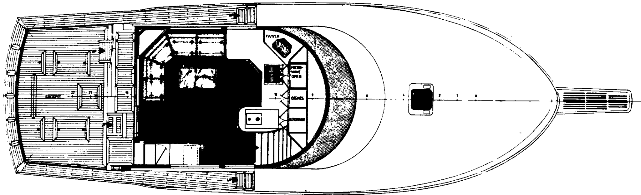
ARRANGEMENT PLAN-SALOON/GALLEY
