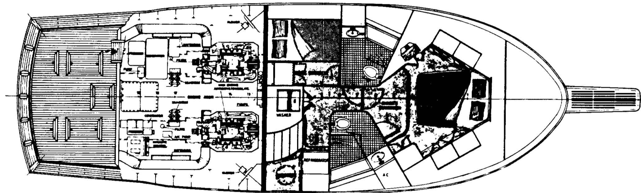
PARTIAL ARRANGEMENT AND ENGINE ROOM
