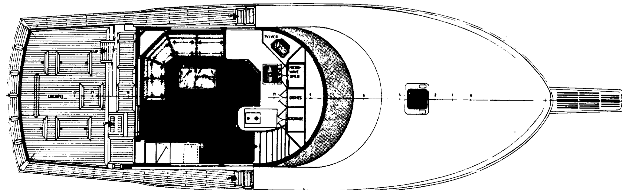
ARRANGEMENT PLAN-SALOON/GALLEY
